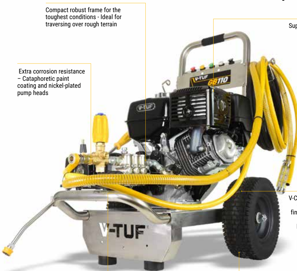
Electric start option GB110SSE – For easy starting in confined spaces
